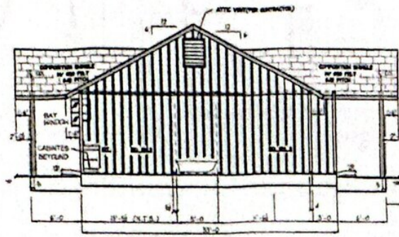
LEFT VIEW
